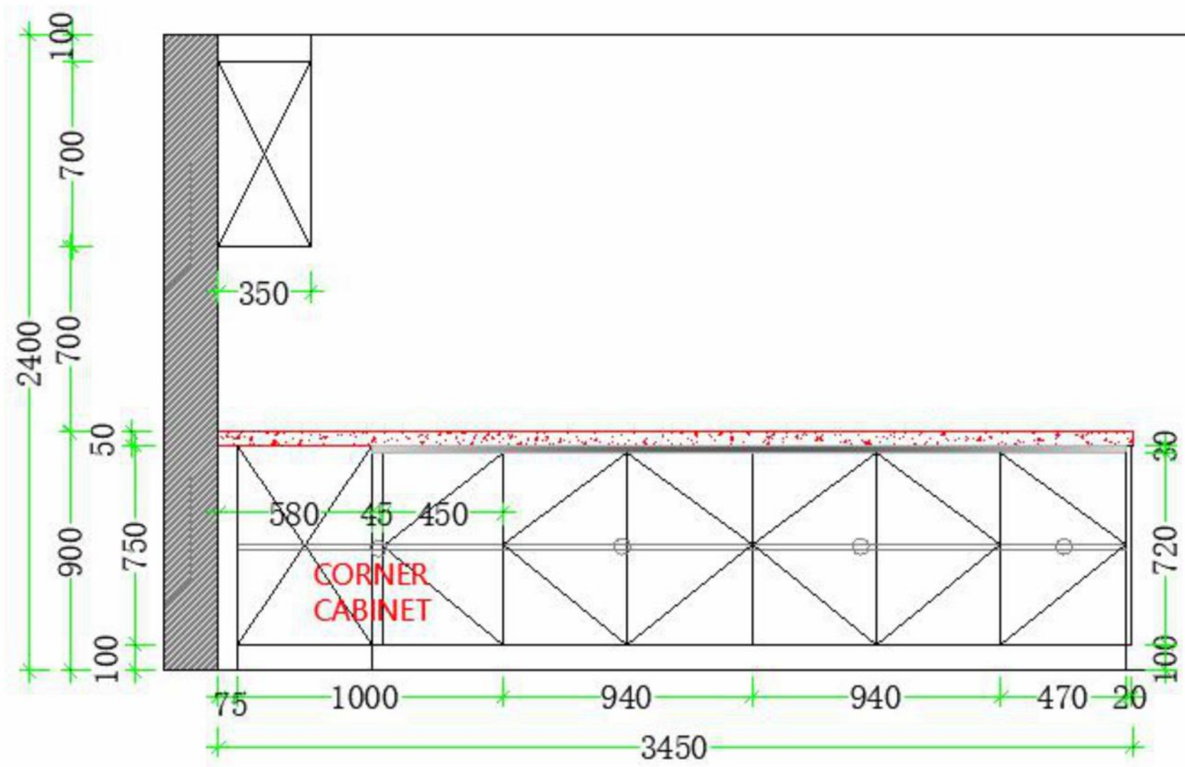
ELEVATION C
