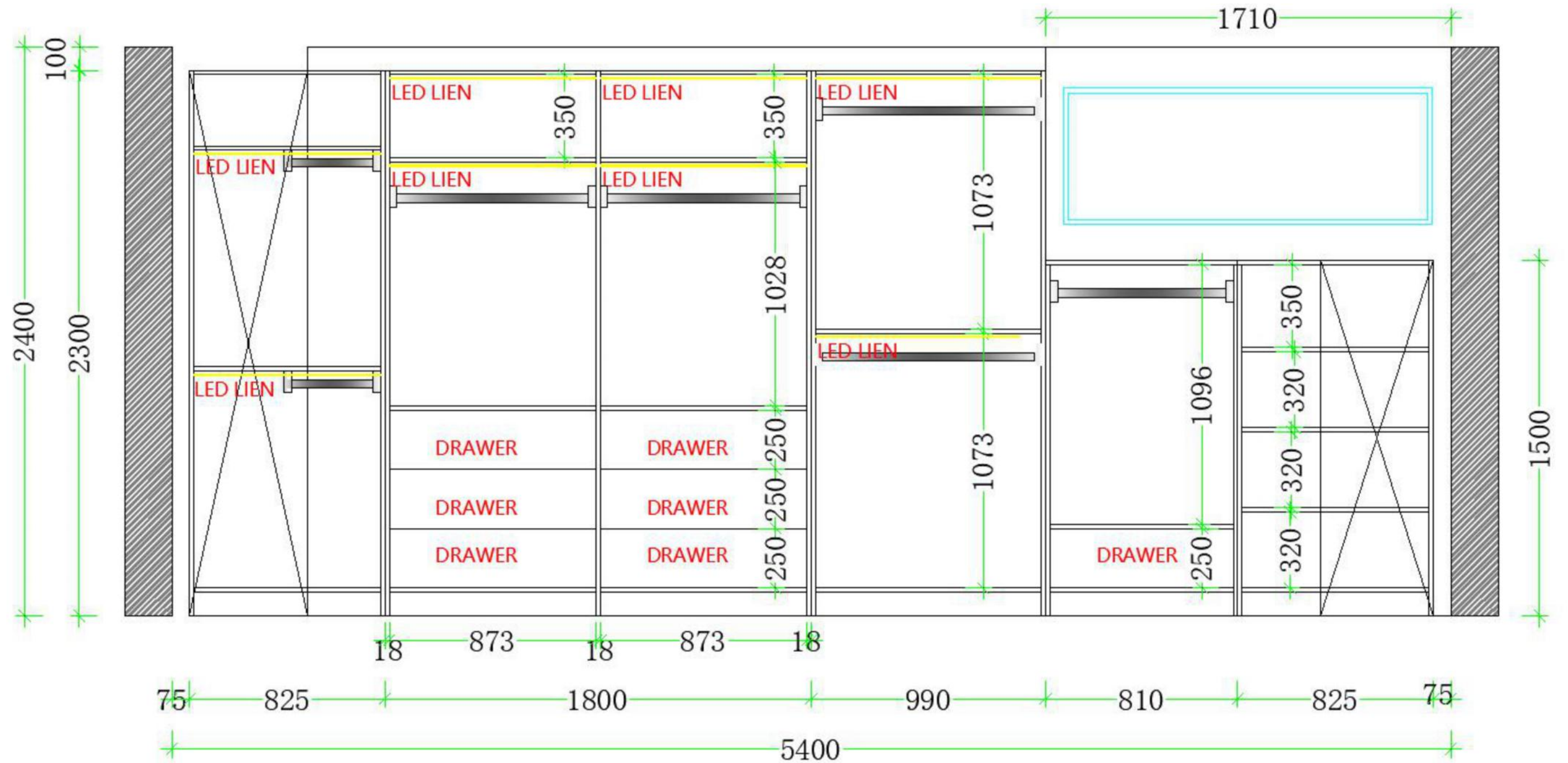
ELEVATION C
